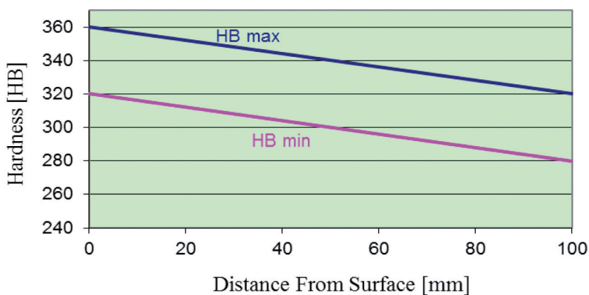
Hardness penetration of the rolls, material V210
