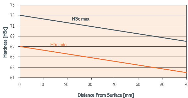
Hardness penetration of the rolls, material B11
